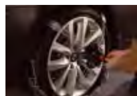
Fitting step 3 Activate the ratchet system to make the chain move toward the rim. The chain will slip automatically onto the tyre when the wheel rotates.
